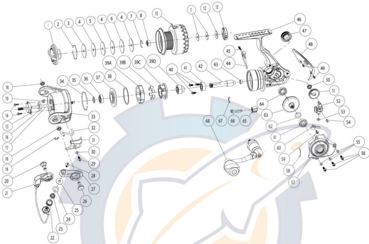
Quantum Catalyst Inshore CI20PTsB Spinning Reel Part List
